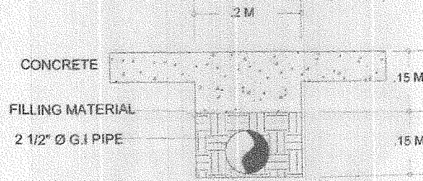
2 DETAIL OF EXCAVATION F-02 RES
