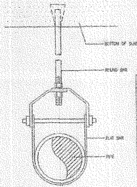
1 ADJUSTABLE CLEVIS PIPE HANGER F-02 RES
